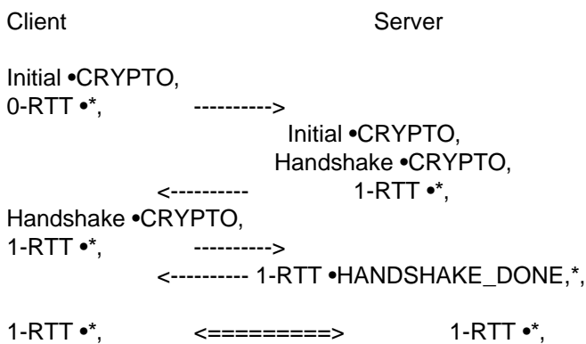
Figure 4: Simplified QUIC Handshake
